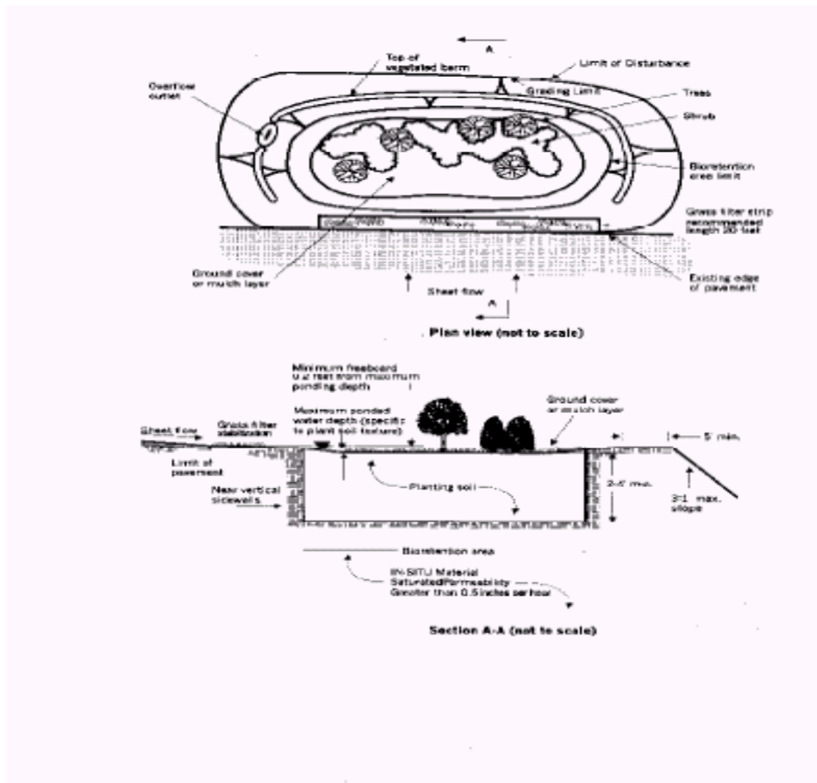
Figure 24-1. Bioretention
