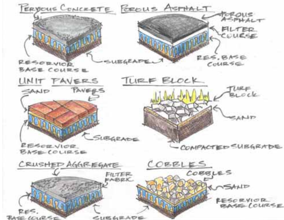
Figure 11-1. Alternative surfaces
