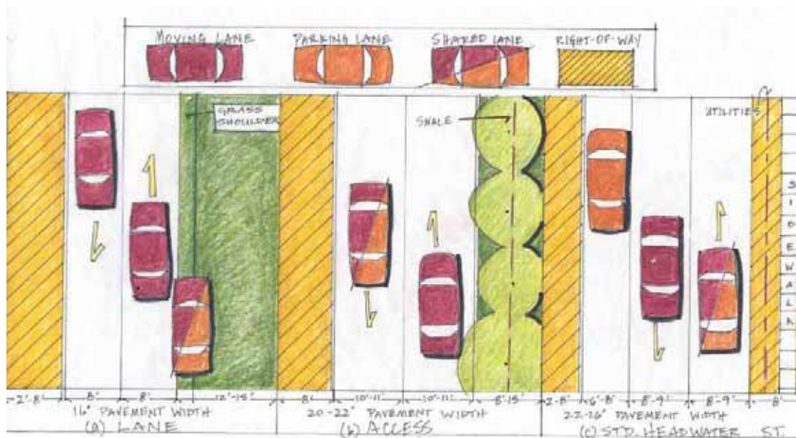
Figure 19-1. Narrow roadways
